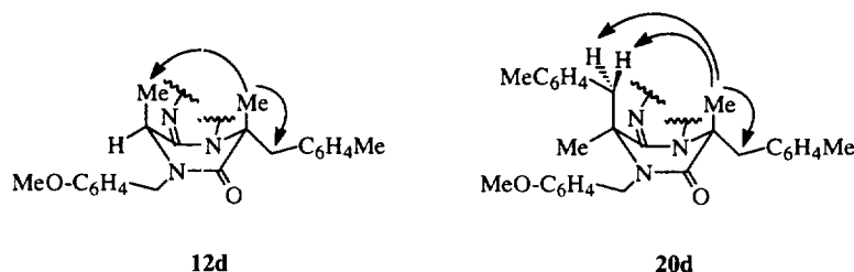
Fig. 3. NOEs registered on 12d and 20d
