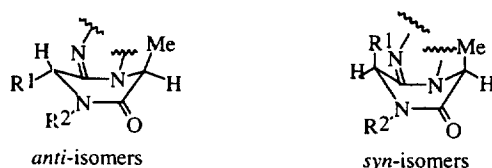
Fig. 2. Conformation of the piperazine ring in 1,4-dialkyl anti - and syn -isomers
